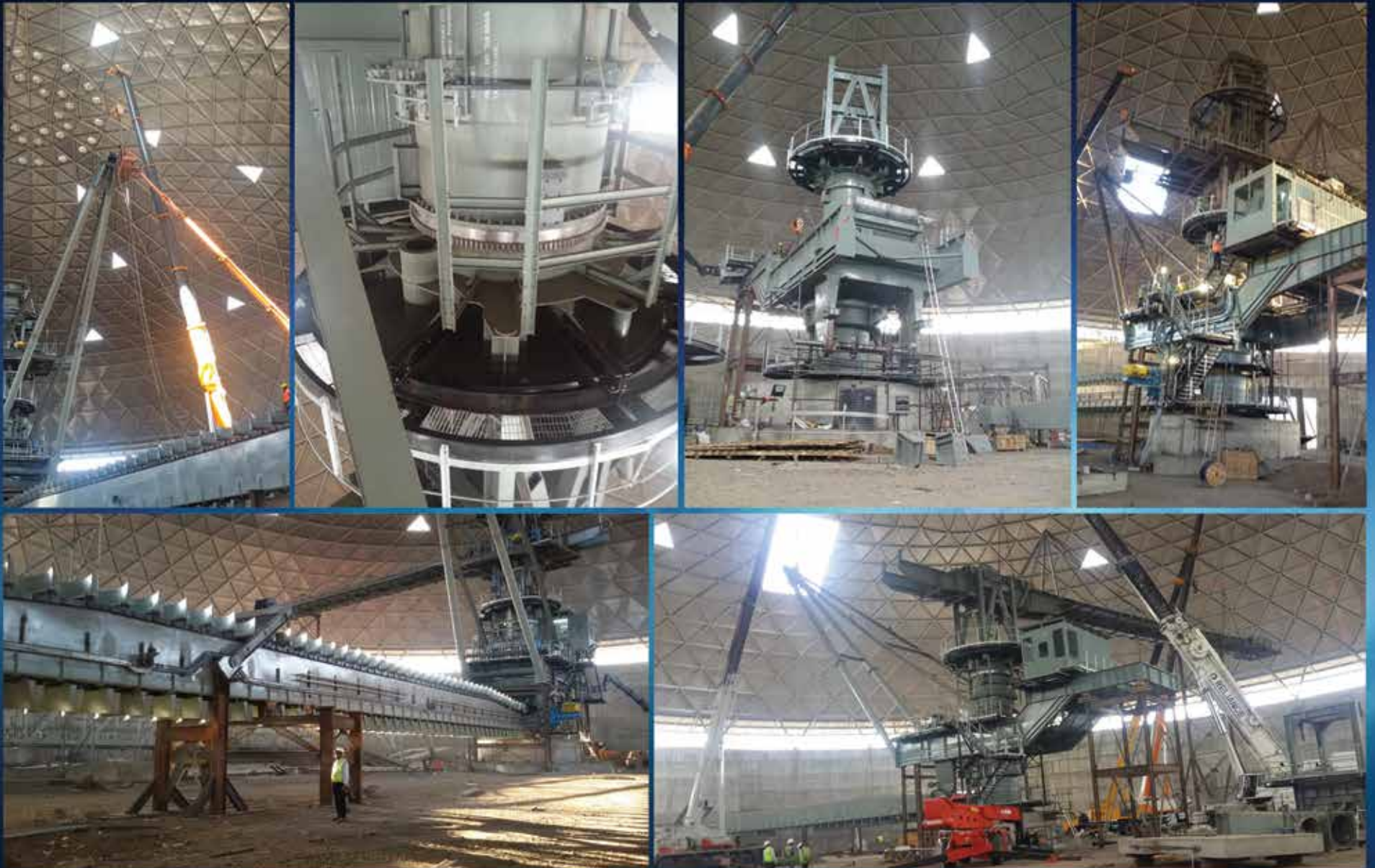
Circular Stacker Reclaimer for Coke Storage Erected at Reliance Refinery, Gujrat, India
